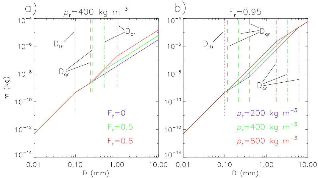
FIG. 1. Examples of the ice particle m – D relationship across the range of particle sizes (solid colored lines): (a) relationship for three different values of F_r (0, 0.5, 0.8) assuming constant \rho_r = 400 \text{ kg m}^{-3} and (b) relationship for three different values of \rho_r (200, 400, 800 \text{ kg m}^{-3} ) assuming constant F_r = 0.95 . Vertical lines show the critical sizes separating small spherical ice from dense nonspherical (or unrimed ice) ice ( D_{th} ; dotted black lines), dense nonspherical ice from graupel ( D_{gr} ; colored dashed lines), and graupel from partially rimed crystals ( D_{cr} ; colored dotted-dashed lines). The colors for D_{gr} and D_{cr} correspond to the given F_r and \rho_r , indicated in the plots ( D_{th} is independent of F_r and \rho_r ).
