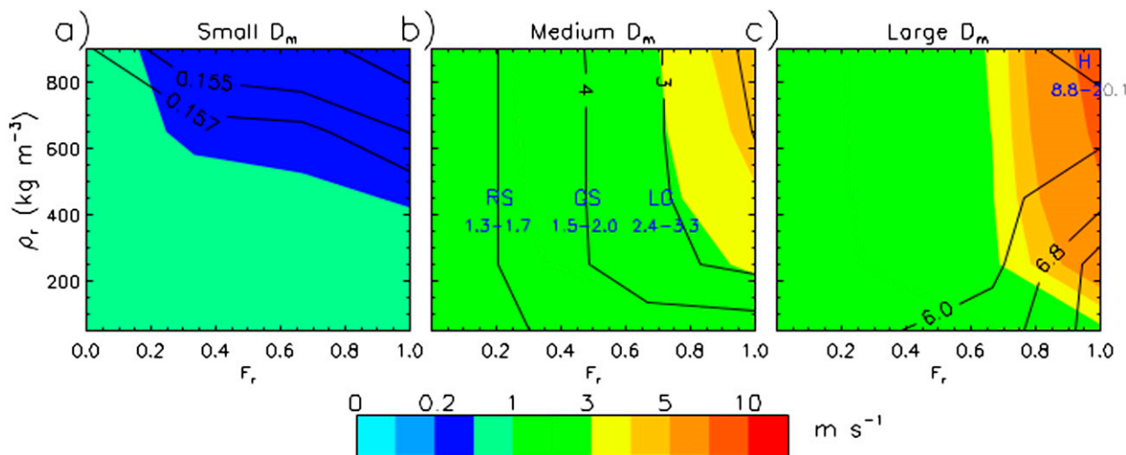
FIG. 2. Mass-weighted bulk ice fall speed as a function of F_r and \rho_r for (a) small D_m ( \sim 0.15\text{--}0.16 mm), (b) medium D_m ( \sim 2\text{--}5 mm), and (c) large D_m ( \sim 5\text{--}7 mm). Black contour lines represent D_m . Empirical values for rimed snow (RS), graupel-like snow (GS), lump graupel (LG), and hail (H) are shown in blue text in (b) and (c). Calculations are made for a temperature of -20^\circ\text{C} and a pressure of 600 hPa.
